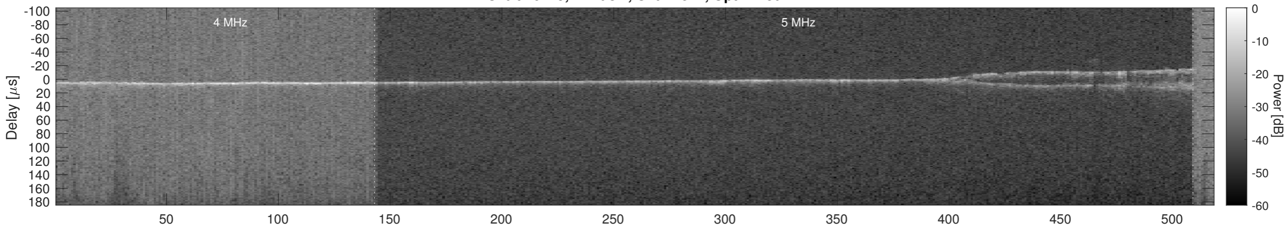
Orbit 20249, Cluttergram
