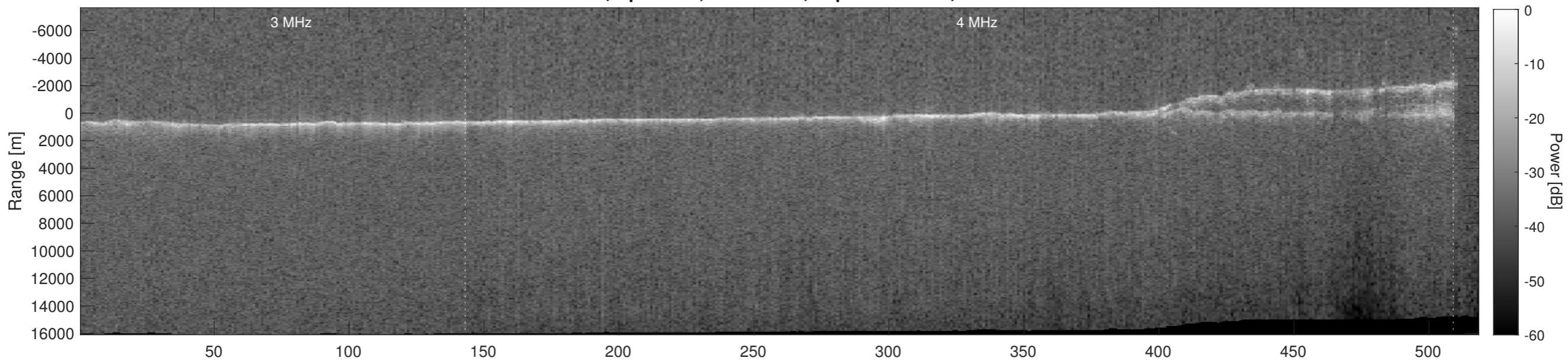
Orbit 20249, Depth-Corrected Cluttergram
