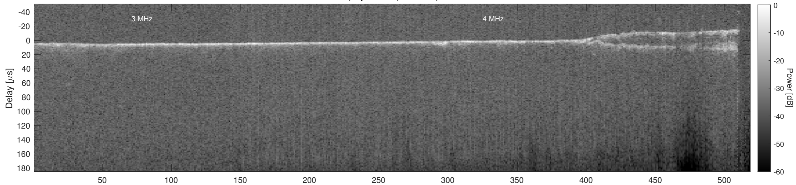
Orbit 20249, Cluttergram
