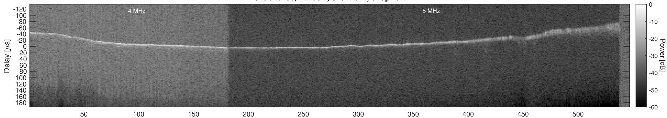
Orbit 20250, Window, Channel 1, Optimized
