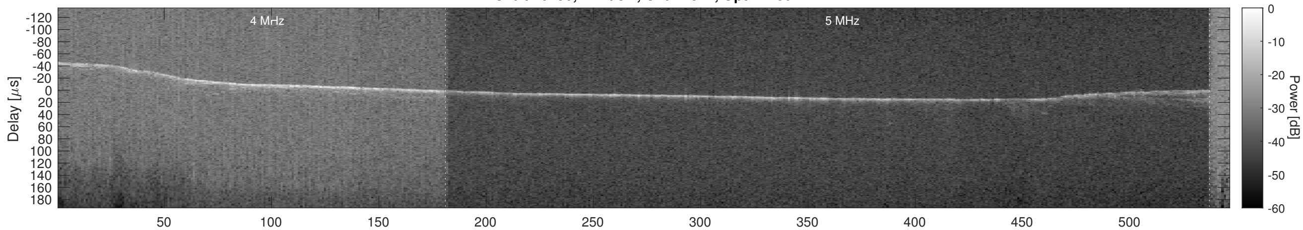
Orbit 20250, Cluttergram
