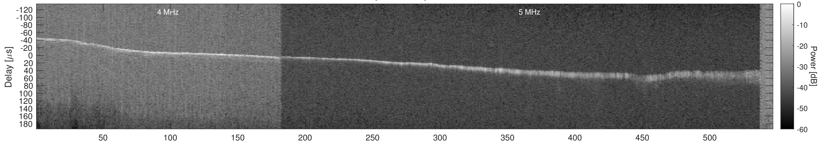
Orbit 20250, Window, Channel 1, Chapman
