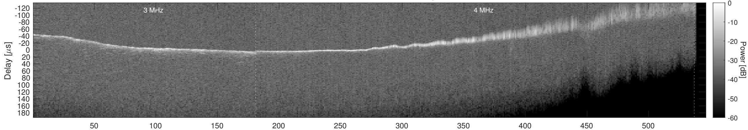
Orbit 20250, Window, Channel 2, Optimized
