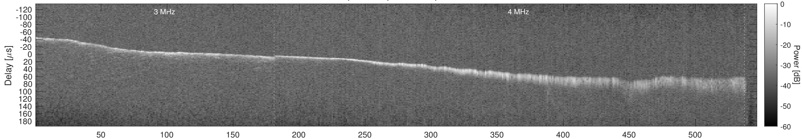
Orbit 20250, Window, Channel 2, Chapman
