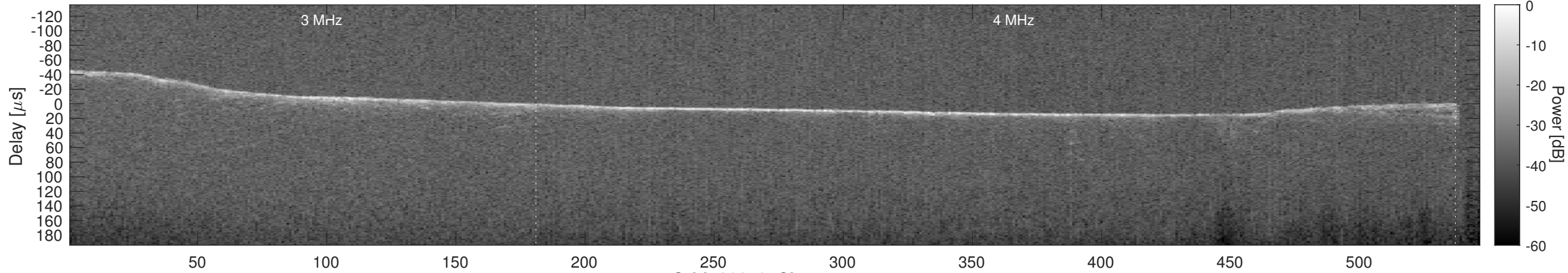
Orbit 20250, Cluttergram
