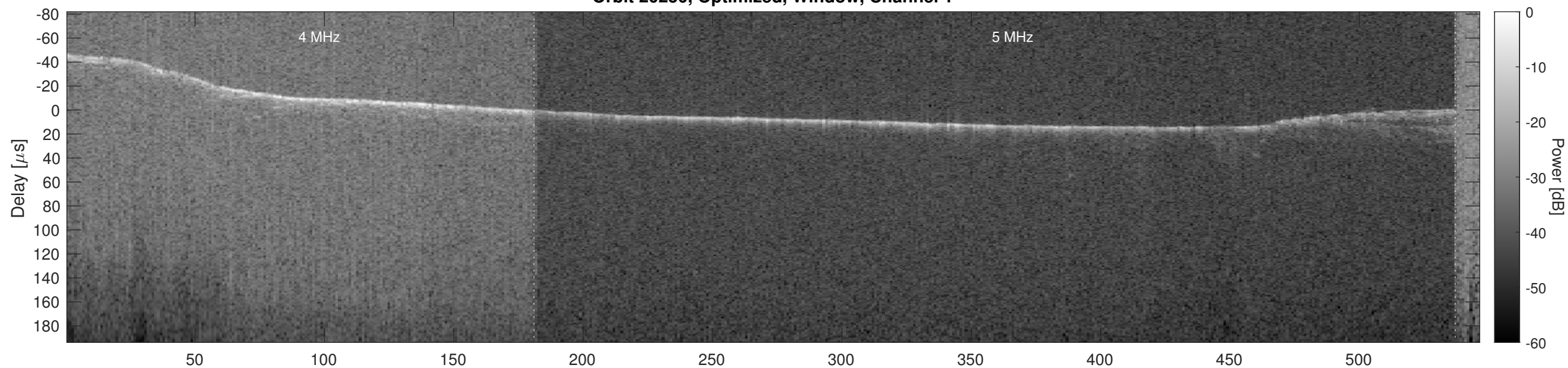
Orbit 20250, Optimized, Window, Channel 2
