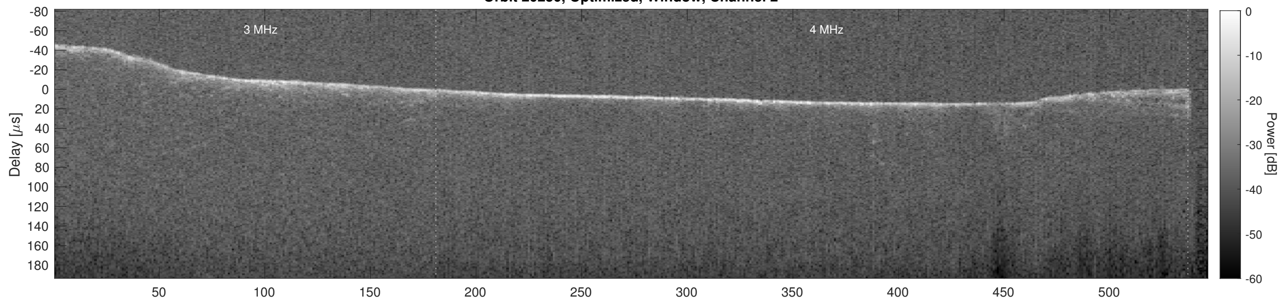
Orbit 20250, Cluttergram
