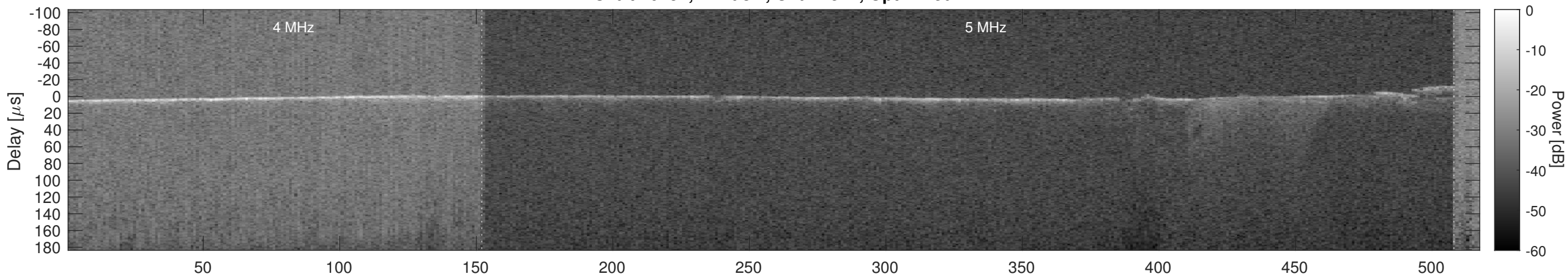
Orbit 20254, Cluttergram
