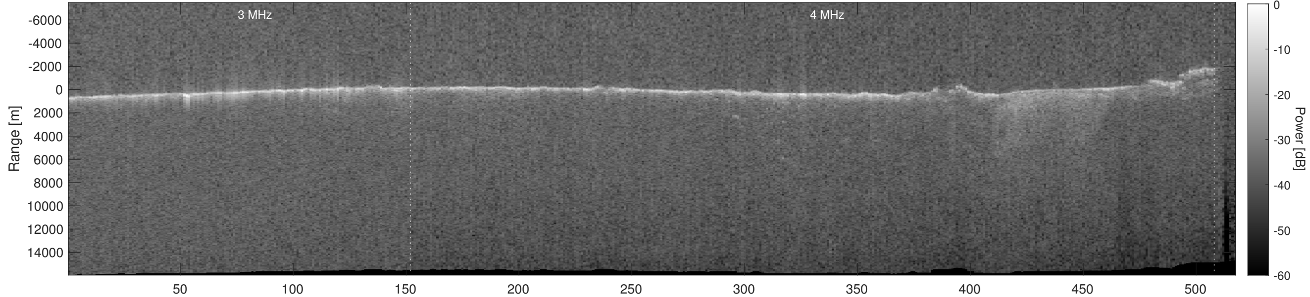
Orbit 20254, Depth-Corrected Cluttergram
