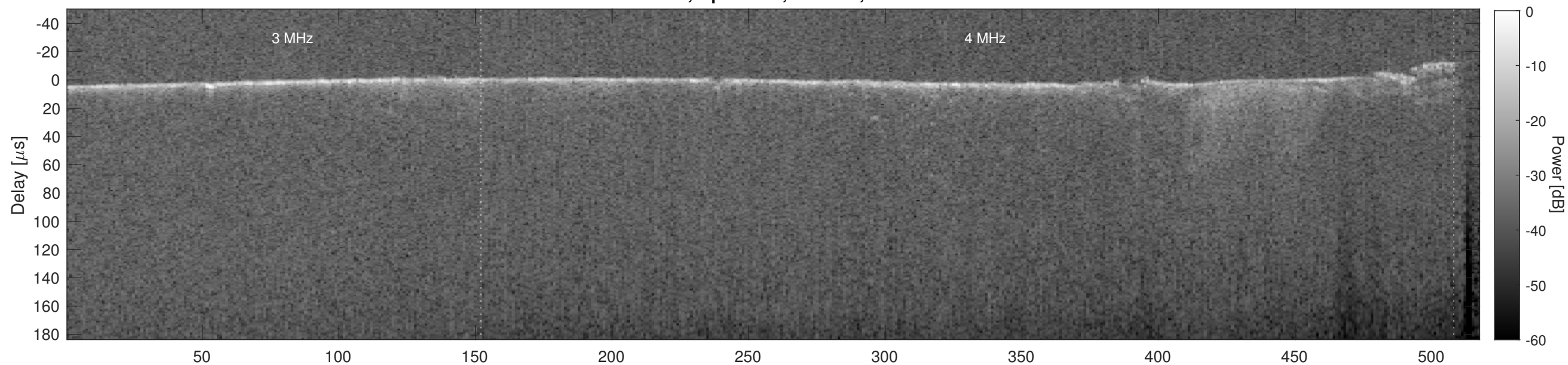
Orbit 20254, Cluttergram
