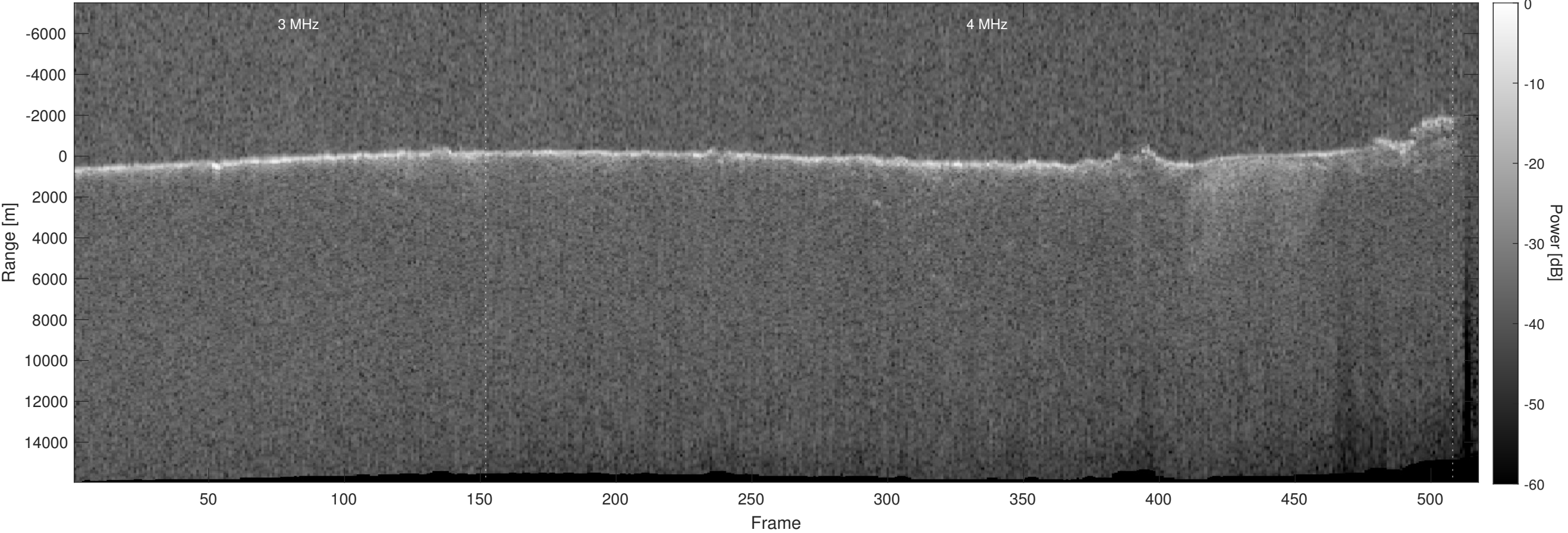
Orbit 20254, Optimized, Window, Depth-Corrected, Channel 2
