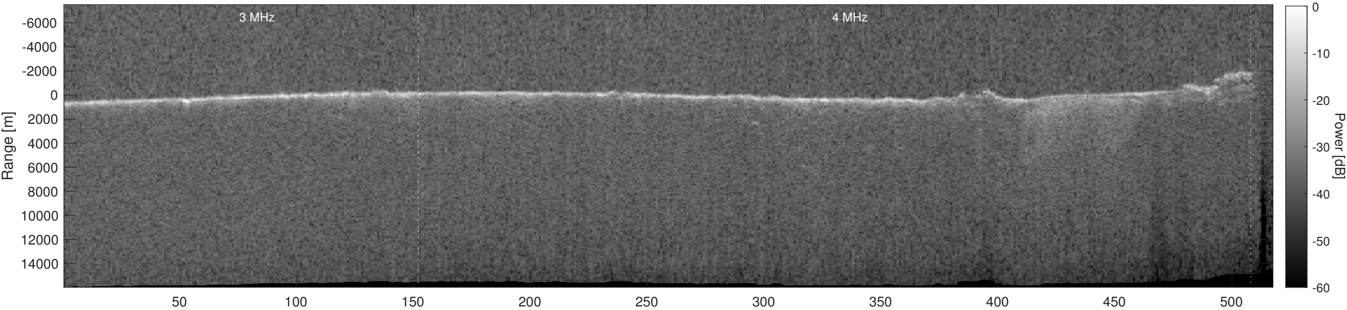
Orbit 20254, Depth-Corrected Cluttergram
