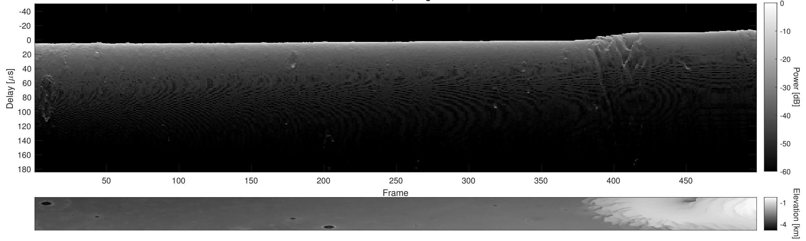
Orbit 20256, Cluttergram
