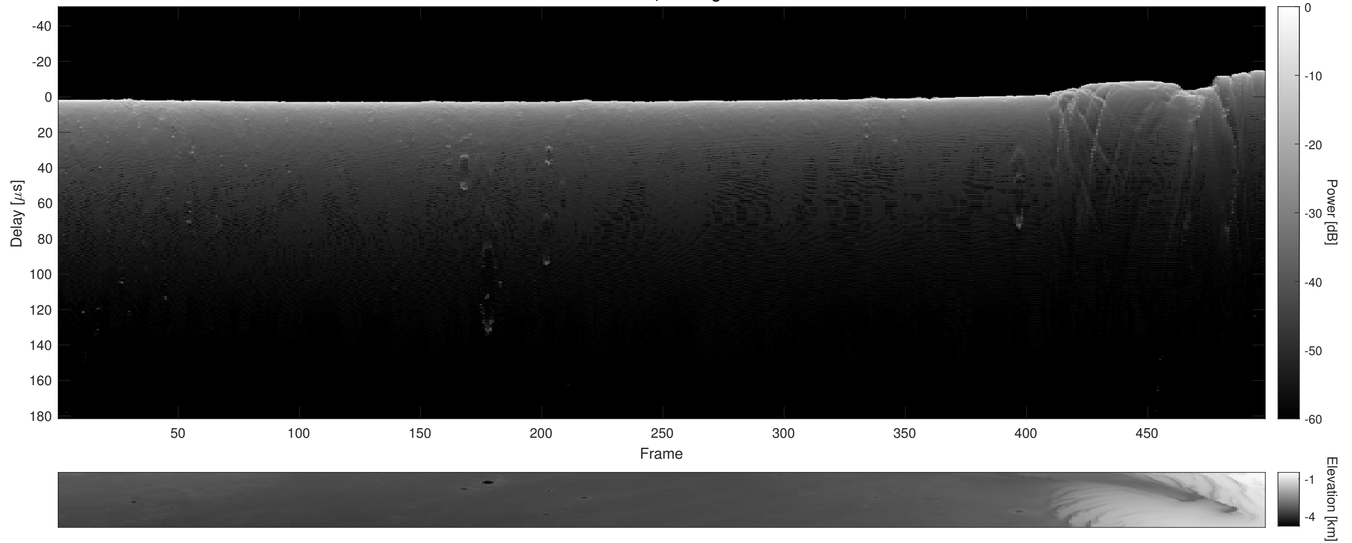
Orbit 20260, Cluttergram
