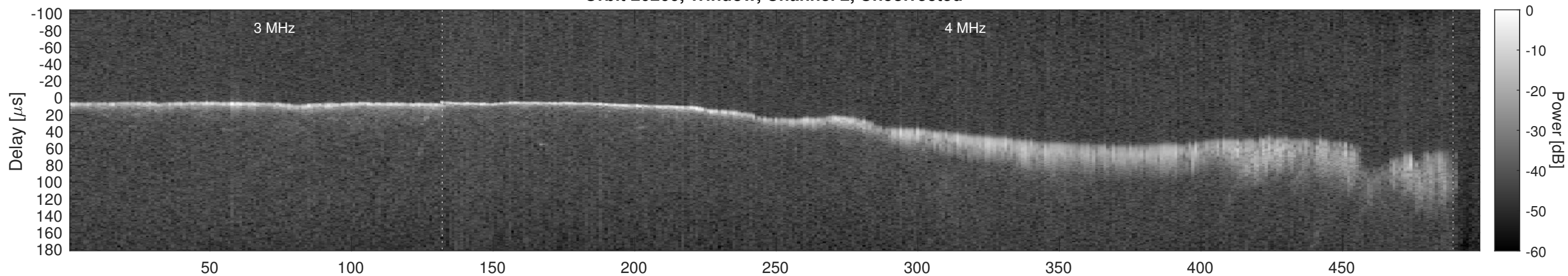
Orbit 20260, Window, Channel 2, Chapman
