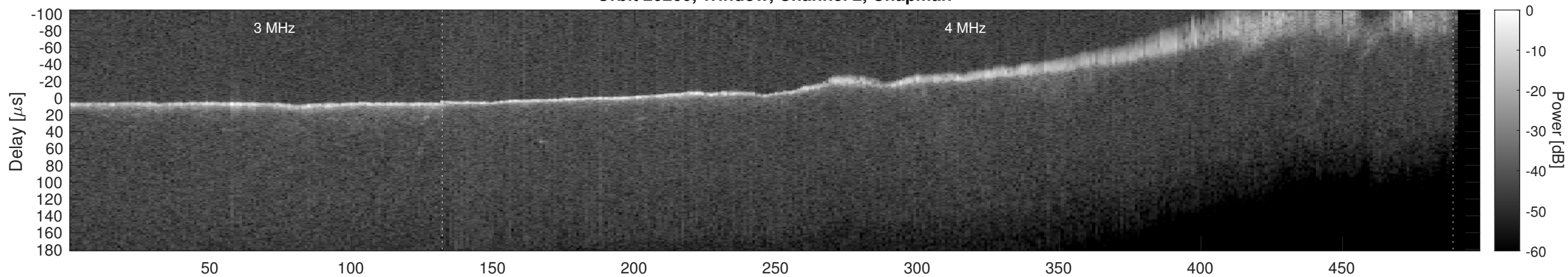
Orbit 20260, Window, Channel 2, Optimized
