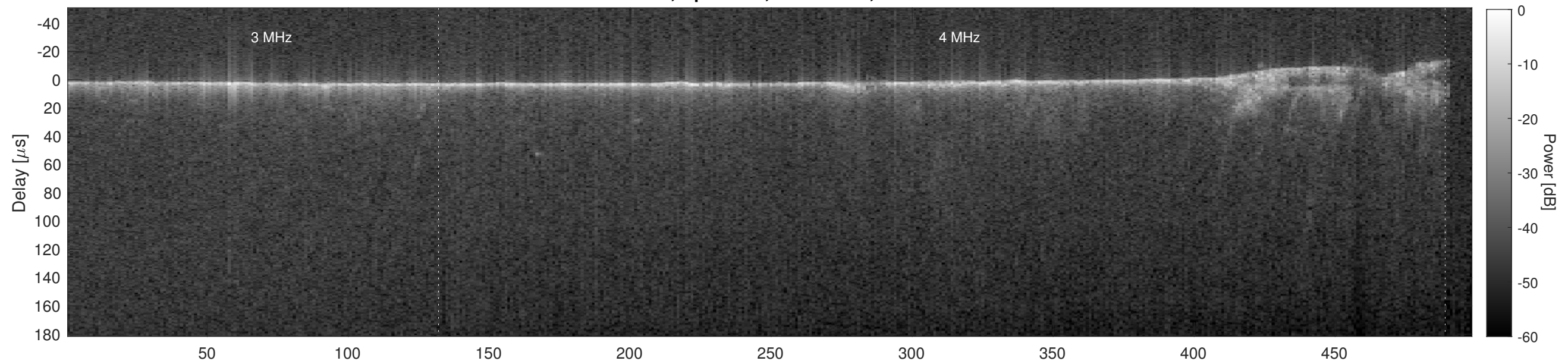
Orbit 20260, Cluttergram
