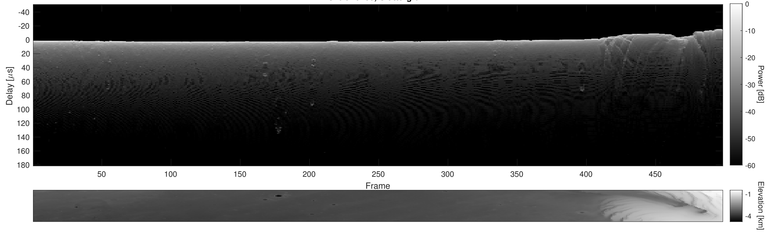
Orbit 20260, Cluttergram
