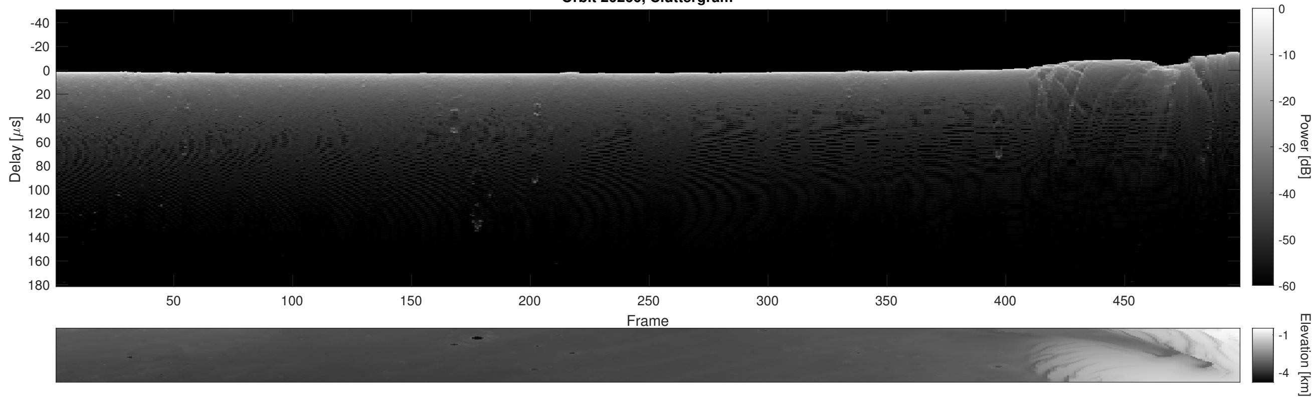
Orbit 20260, Cluttergram
