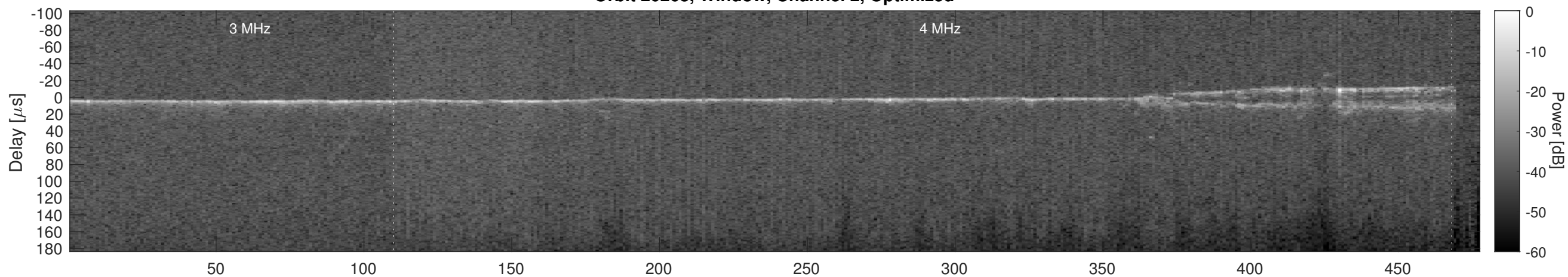
Orbit 20263, Cluttergram
