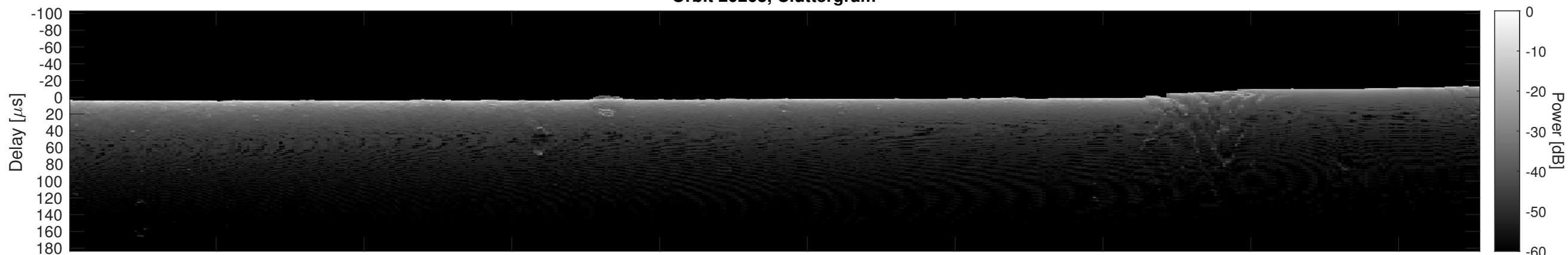
Orbit 20263, Cluttergram
