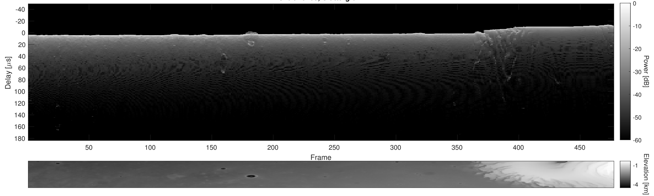
Orbit 20263, Cluttergram
