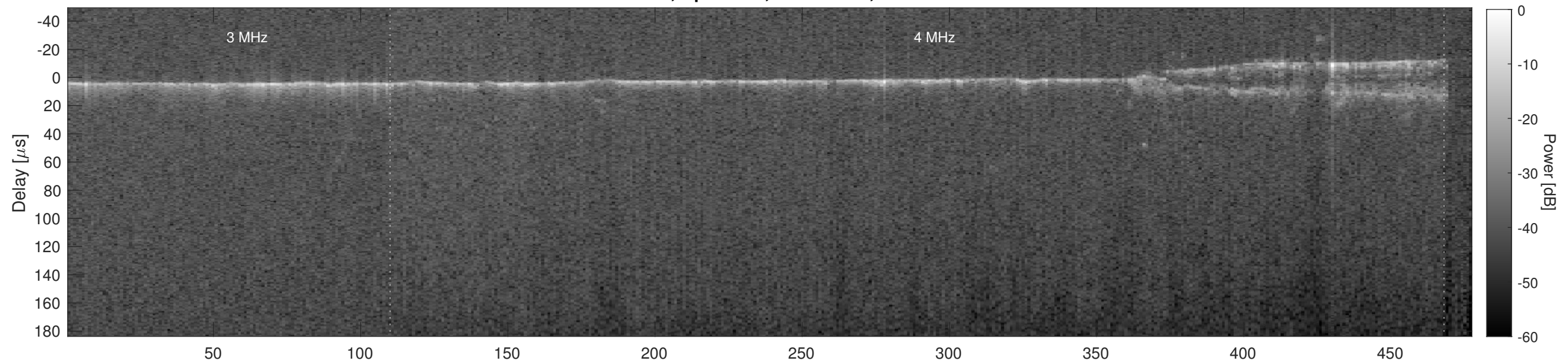
Orbit 20263, Cluttergram
