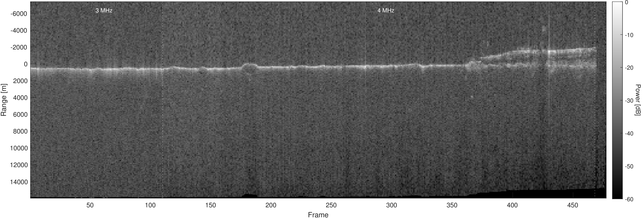
Orbit 20263, Optimized, No Window, Depth-Corrected, Channel 2
