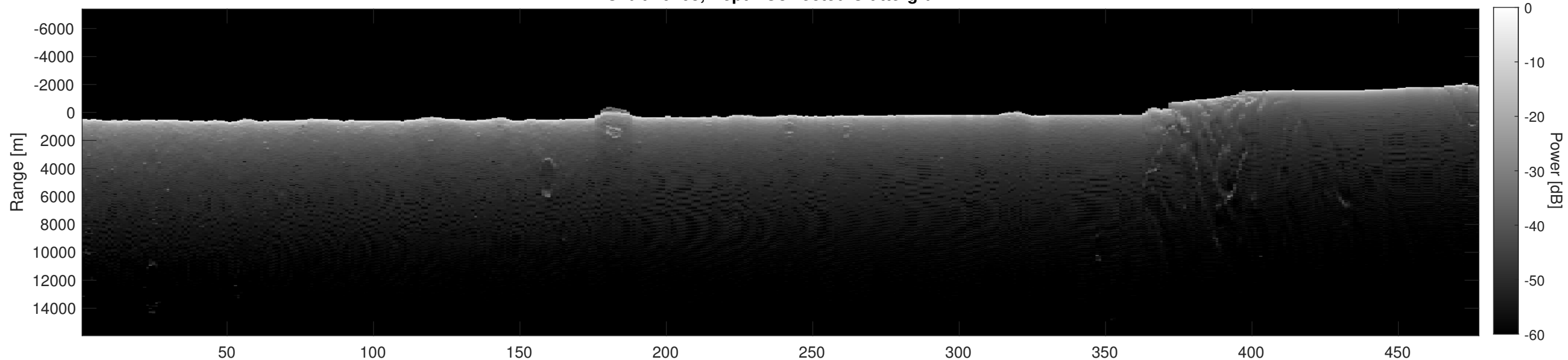
Orbit 20263, Depth-Corrected Cluttergram
