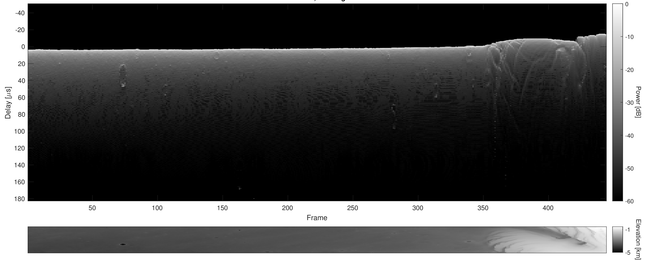
Orbit 20267, Cluttergram
