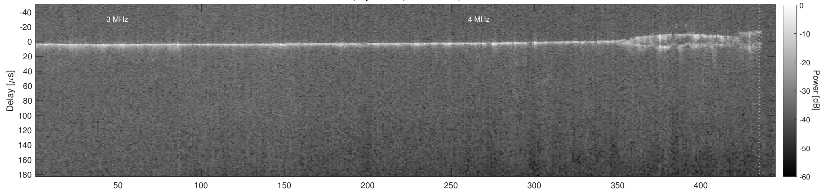
Orbit 20267, Cluttergram
