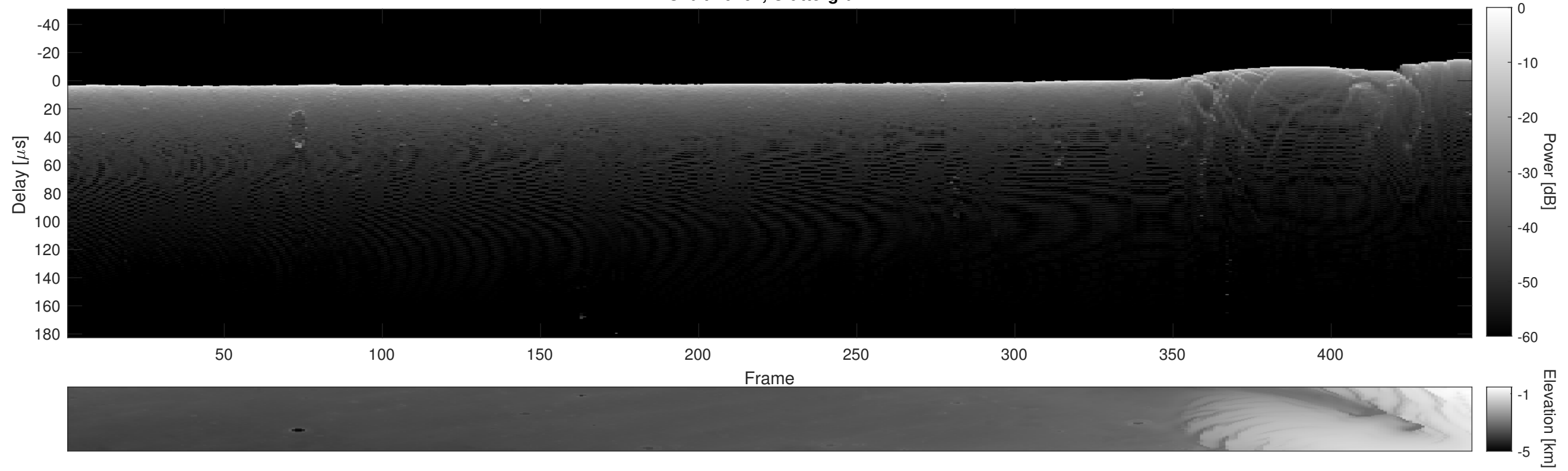
Orbit 20267, Cluttergram
