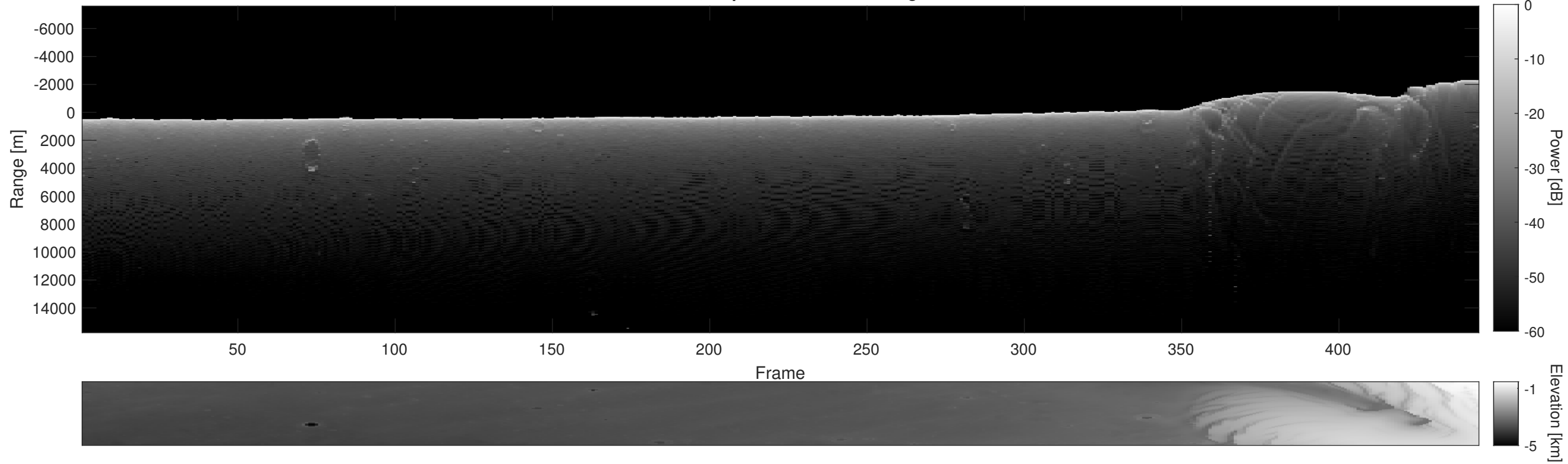
Orbit 20267, Depth-Corrected Cluttergram
