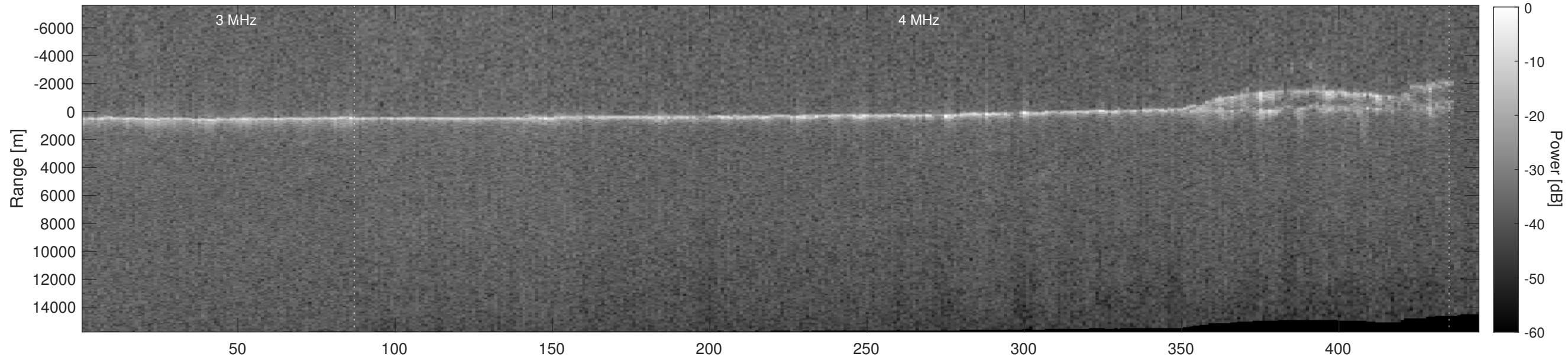
Orbit 20267, Depth-Corrected Cluttergram
