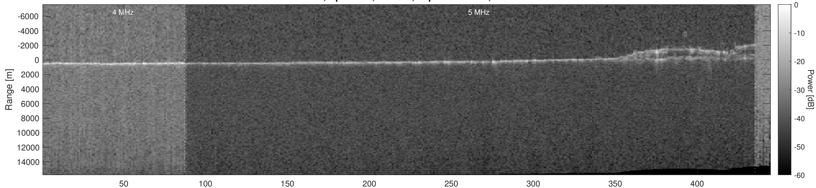
Orbit 20267, Optimized, Window, Depth-Corrected, Channel 2
