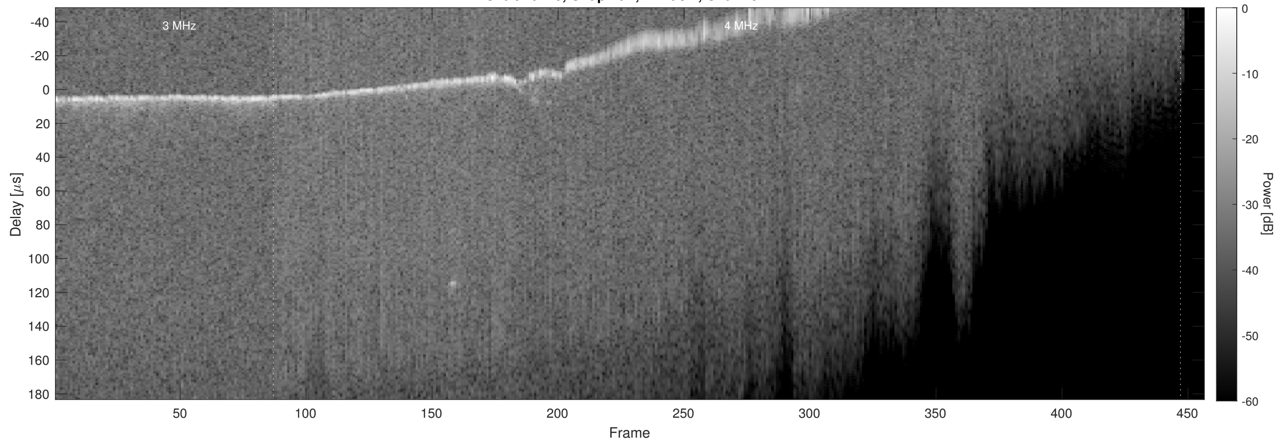
Orbit 20270, Chapman, Window, Channel 2
