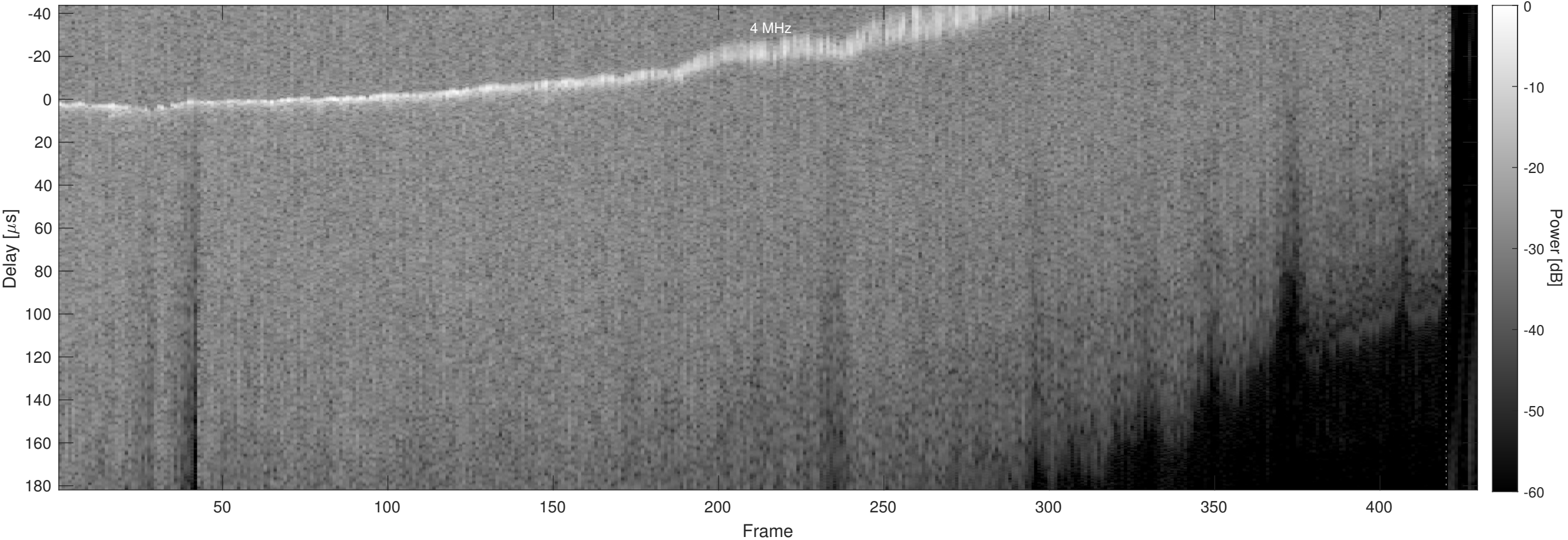
Orbit 20273, Chapman, No Window, Channel 2
