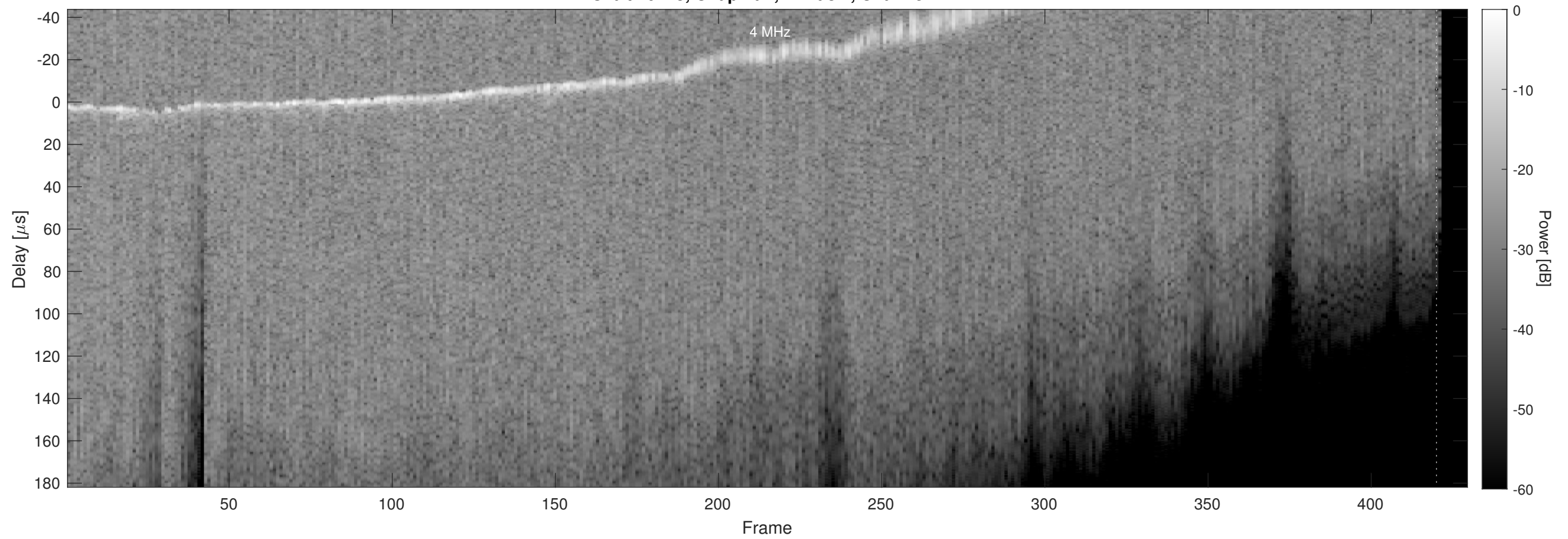
Orbit 20273, Chapman, Window, Channel 2
