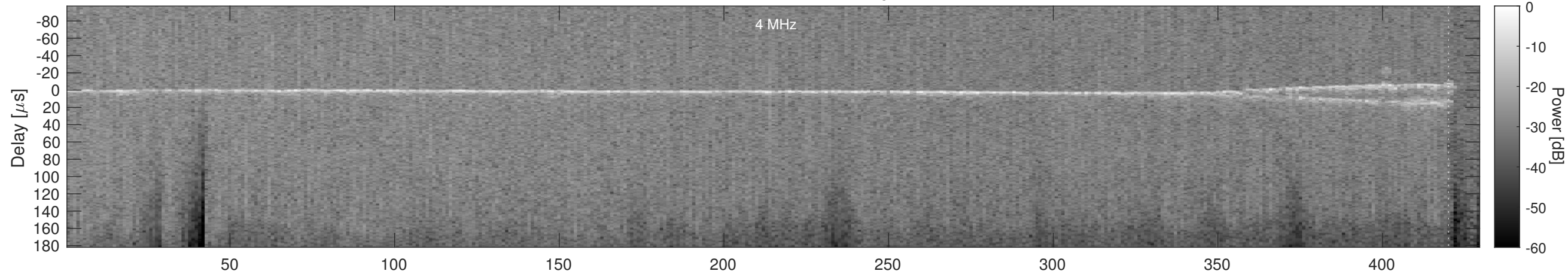
Orbit 20273, Cluttergram
