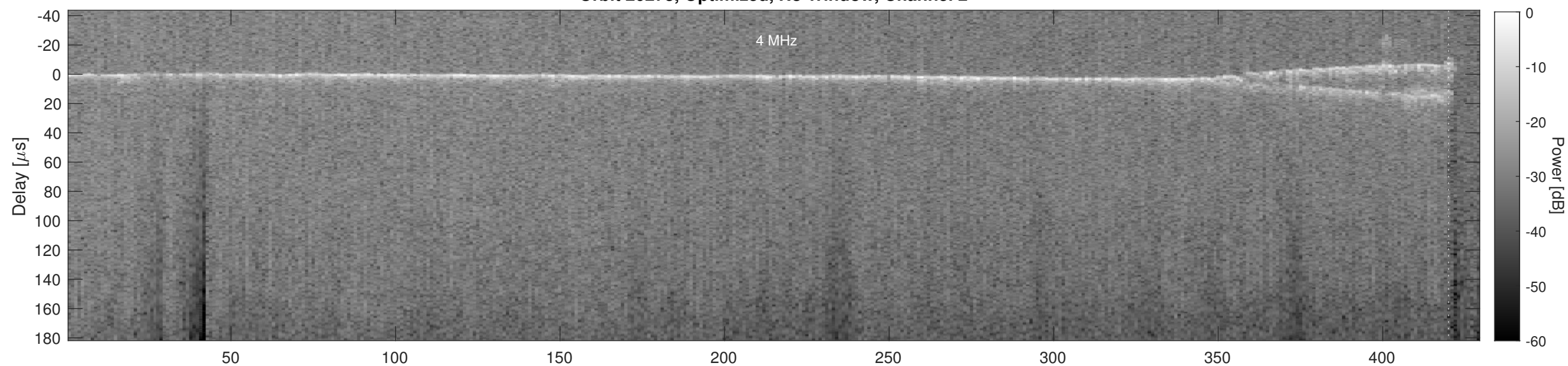
Orbit 20273, Cluttergram
