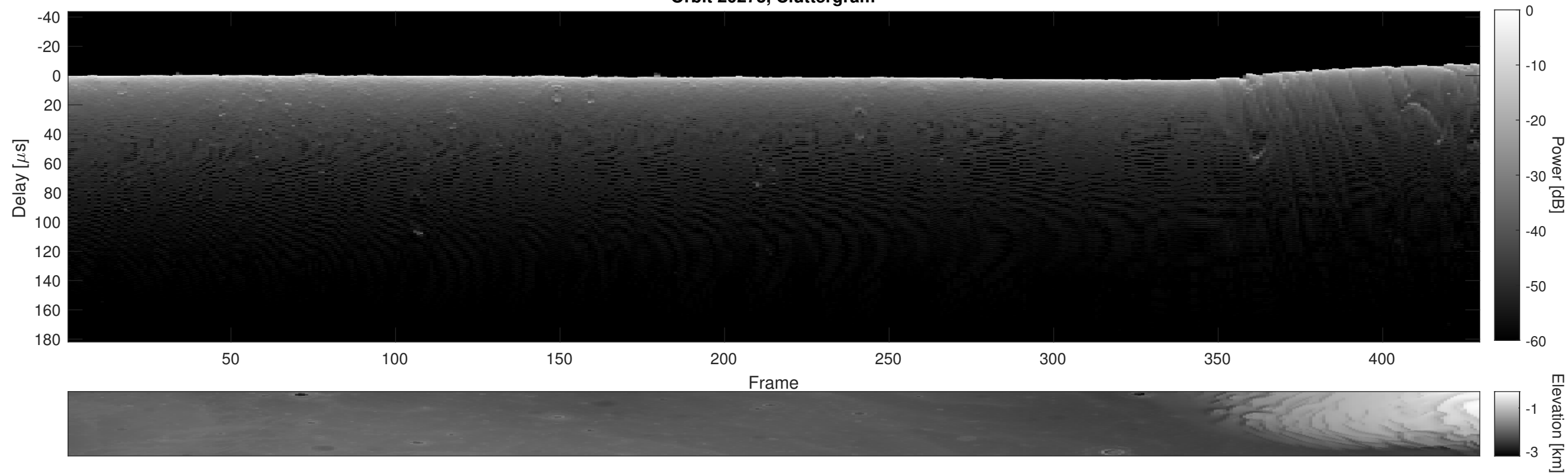
Orbit 20273, Cluttergram
