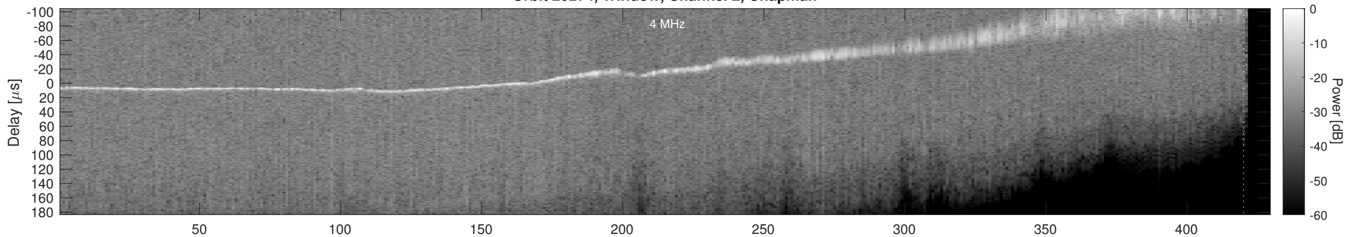
Orbit 20274, Window, Channel 2, Optimized
