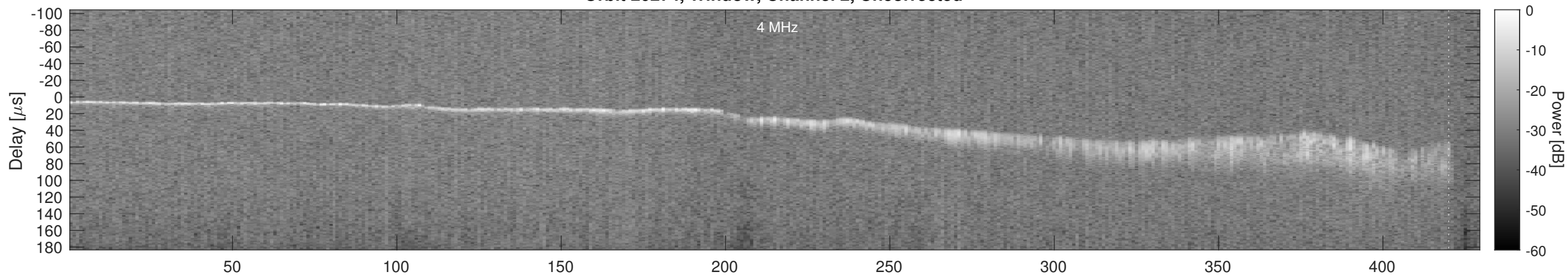
Orbit 20274, Window, Channel 2, Chapman
