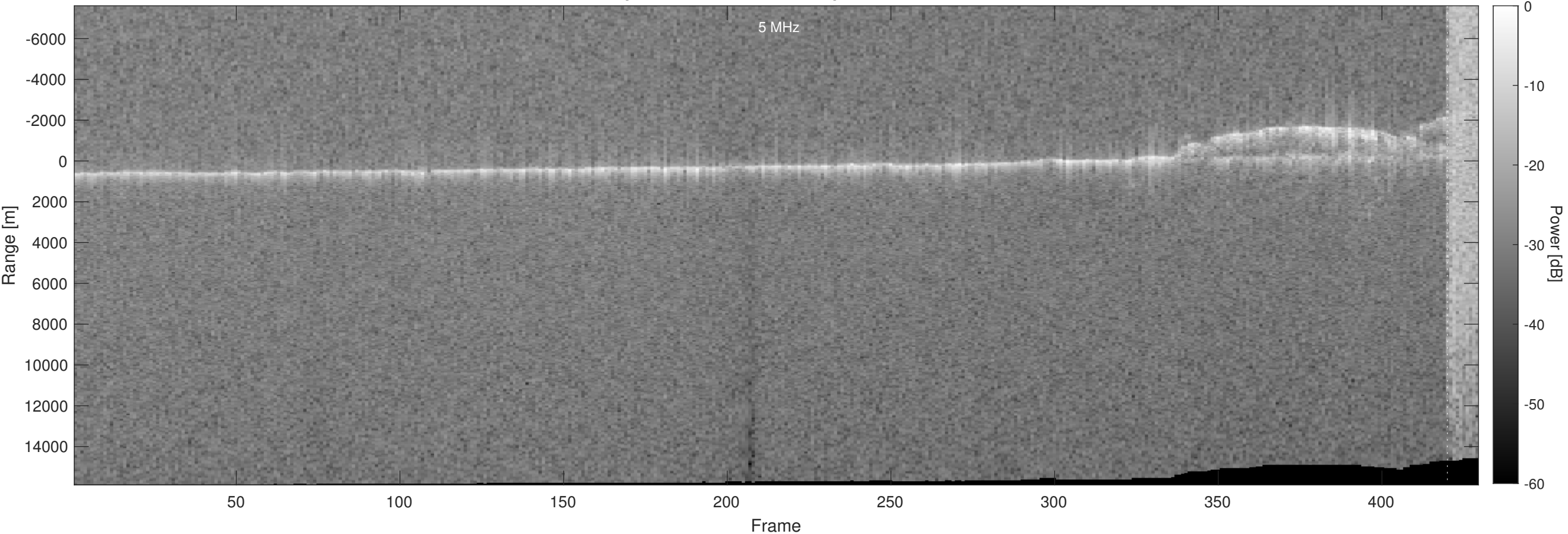
Orbit 20274, Optimized, No Window, Depth-Corrected, Channel 2
