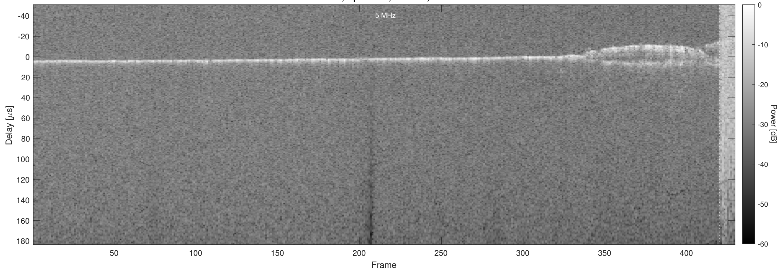
Orbit 20274, Optimized, Window, Channel 2
