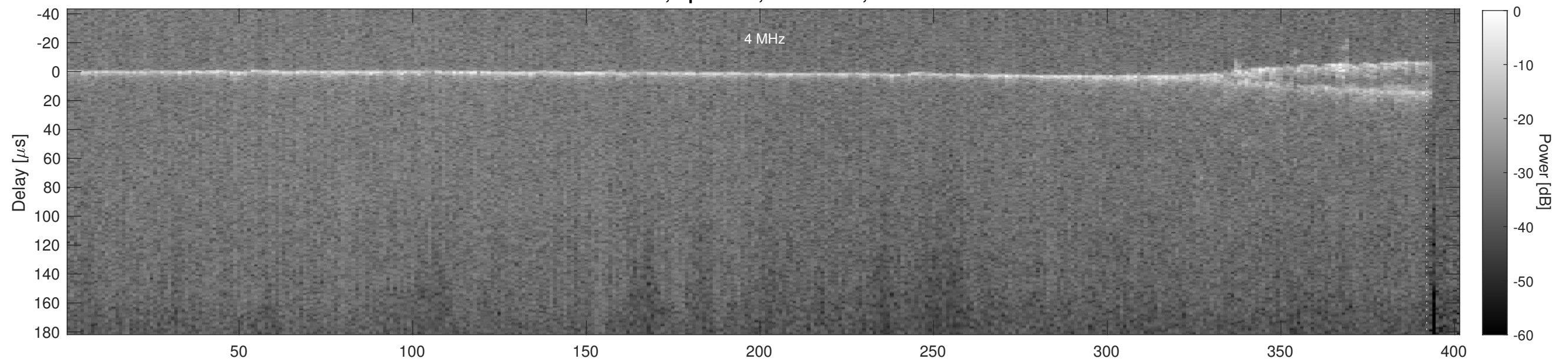
Orbit 20280, Cluttergram
