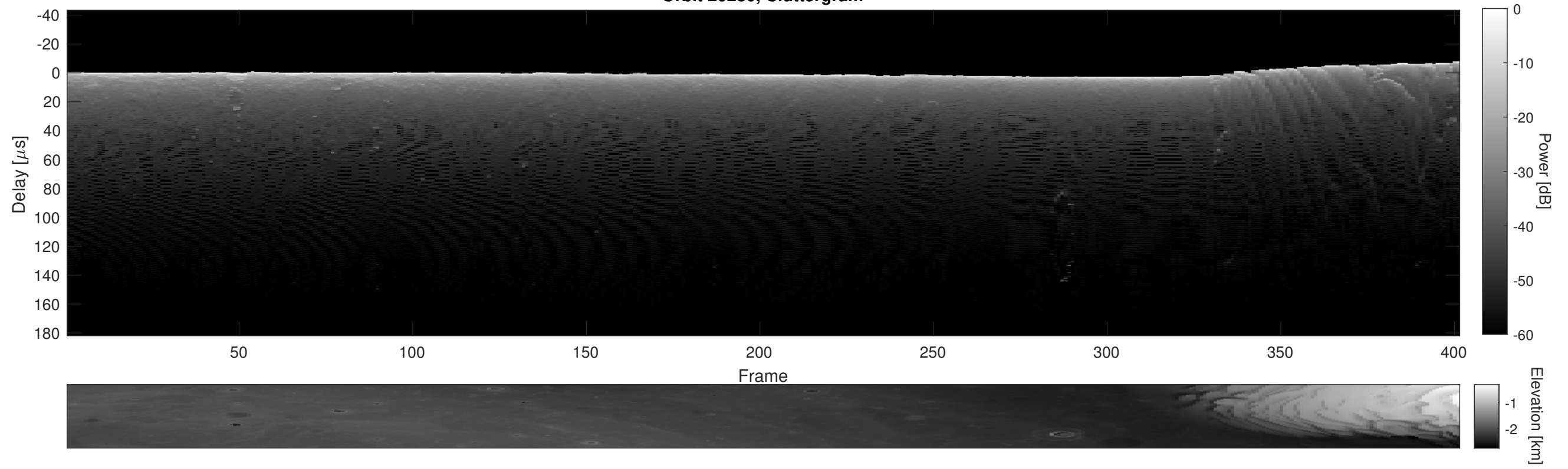
Orbit 20280, Cluttergram
