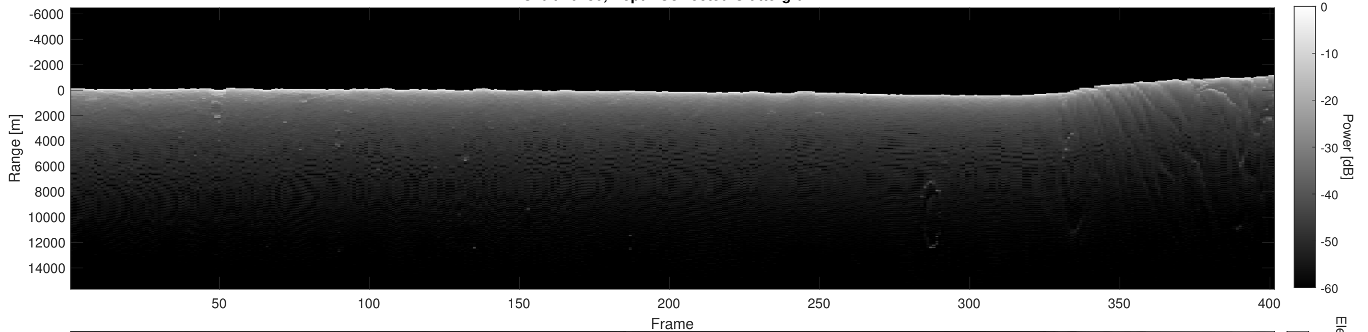
Orbit 20280, Depth-Corrected Cluttergram
