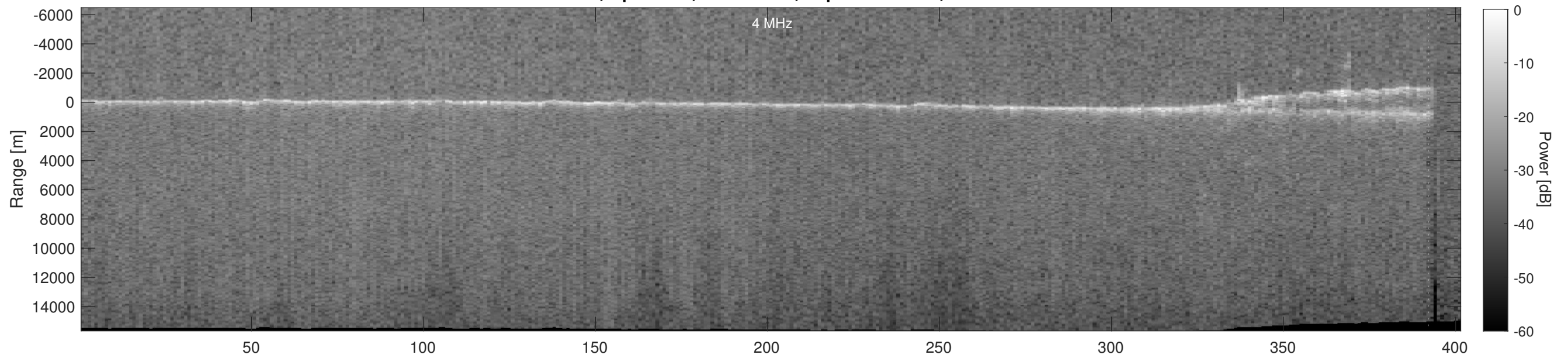
Orbit 20280, Depth-Corrected Cluttergram
