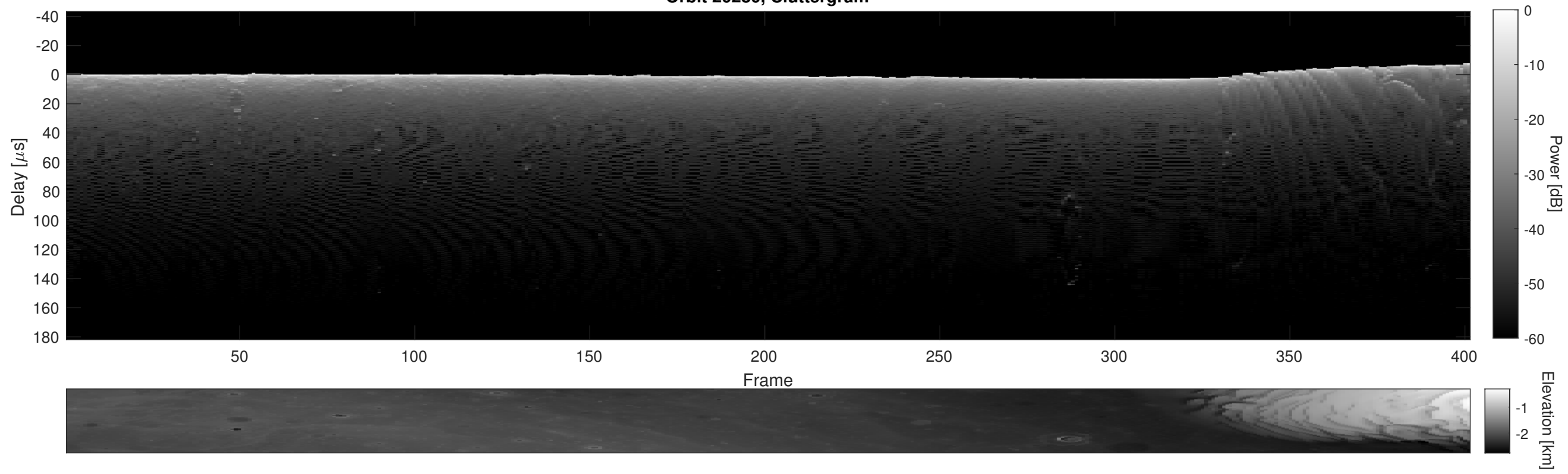
Orbit 20280, Cluttergram
