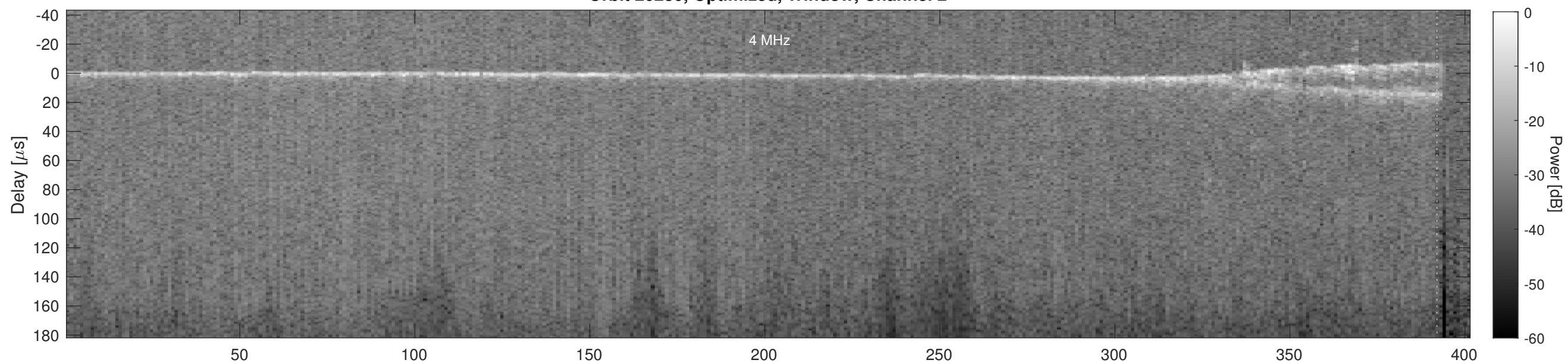
Orbit 20280, Cluttergram
