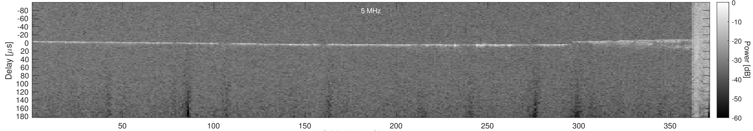
Orbit 20285, Cluttergram
