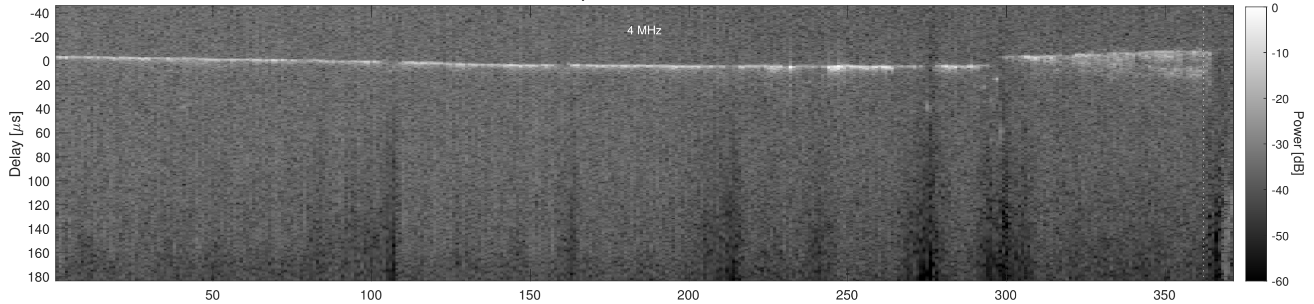
Orbit 20285, Cluttergram
