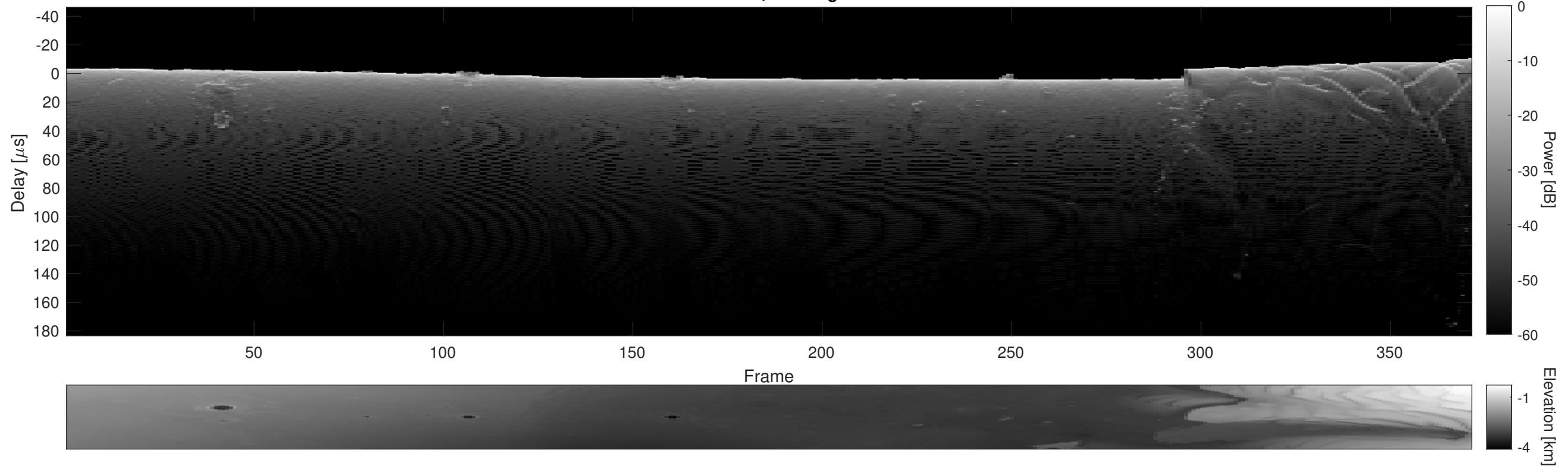
Orbit 20285, Cluttergram
