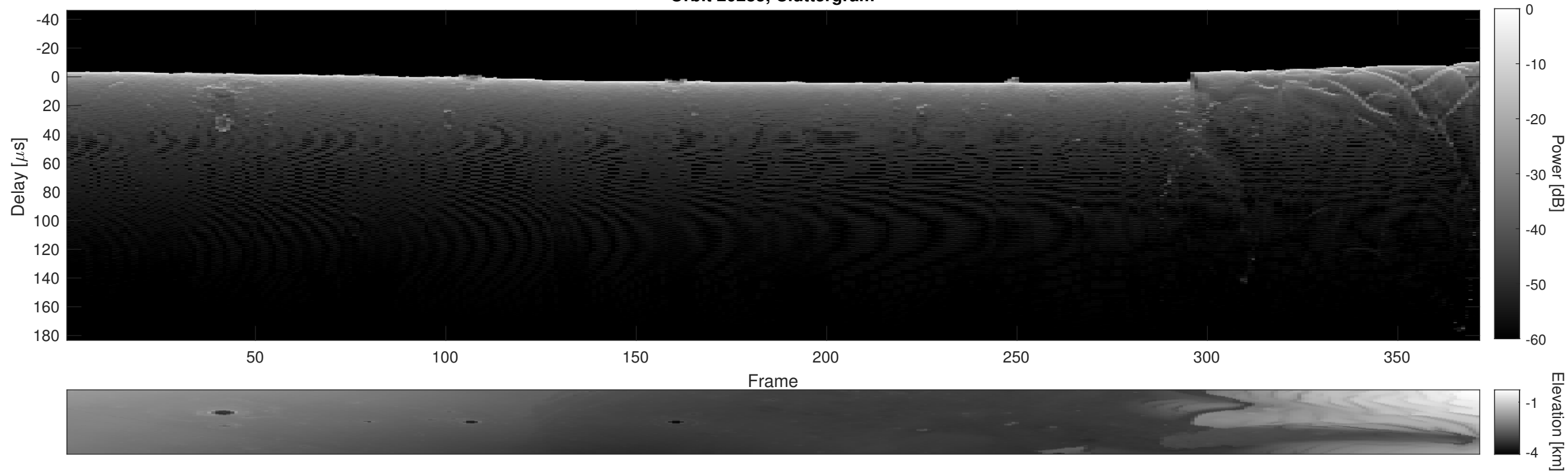
Orbit 20285, Cluttergram
