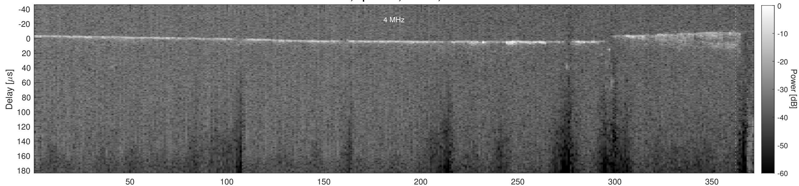
Orbit 20285, Cluttergram
