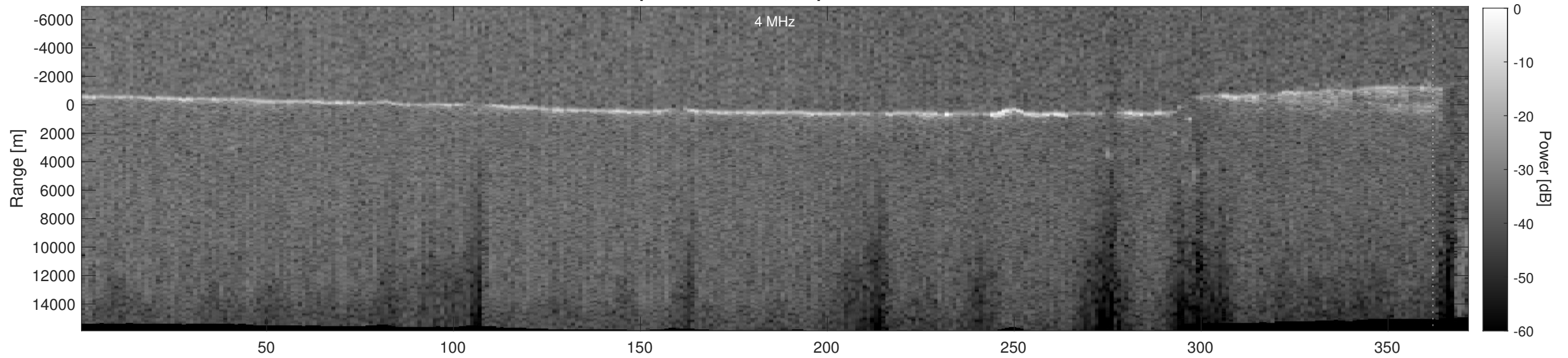
Orbit 20285, Depth-Corrected Cluttergram
