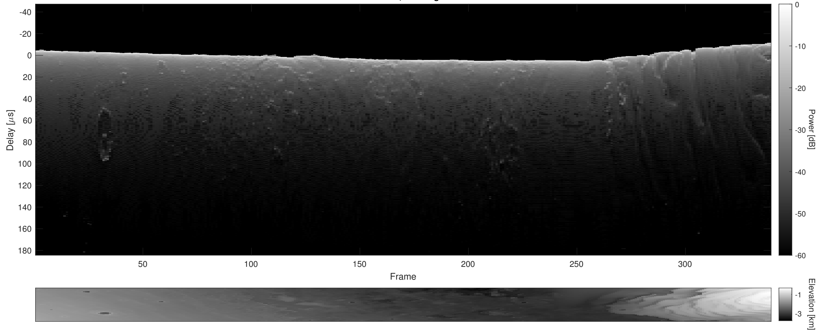
Orbit 20289, Cluttergram
