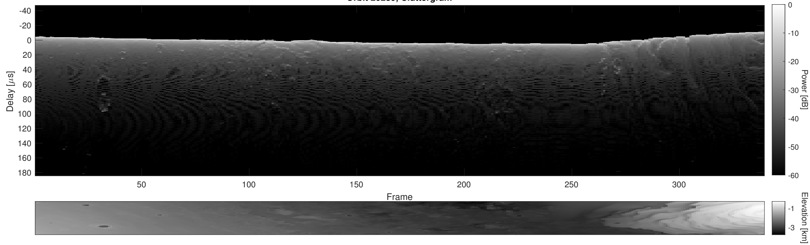
Orbit 20289, Cluttergram
