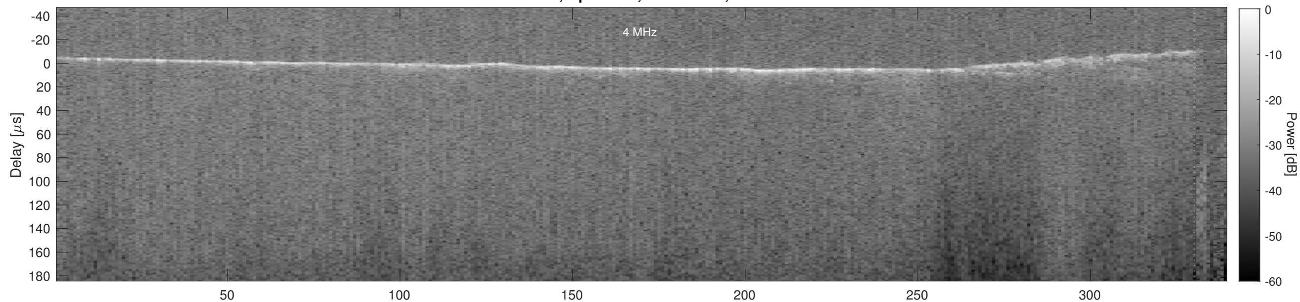
Orbit 20289, Cluttergram
