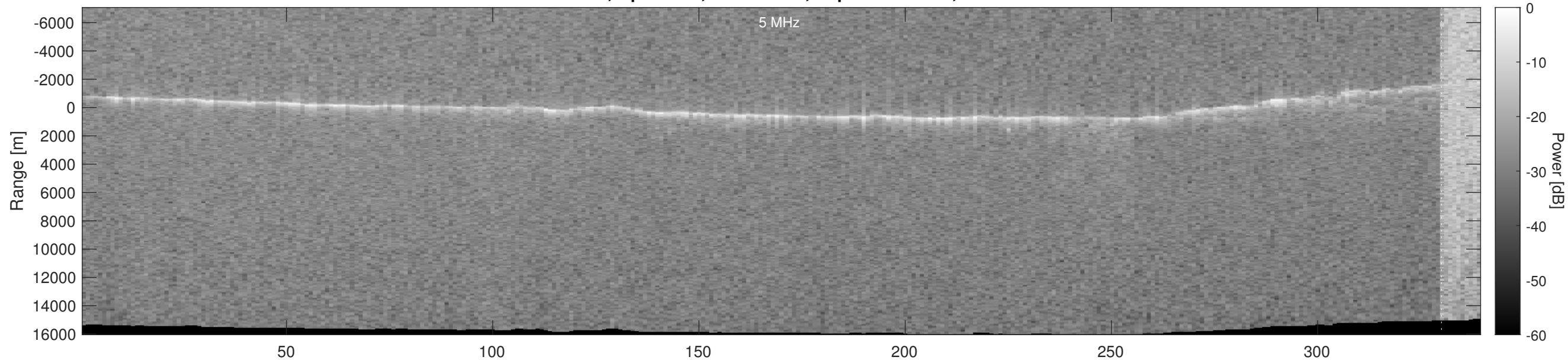
Orbit 20289, Optimized, No Window, Depth-Corrected, Channel 2
