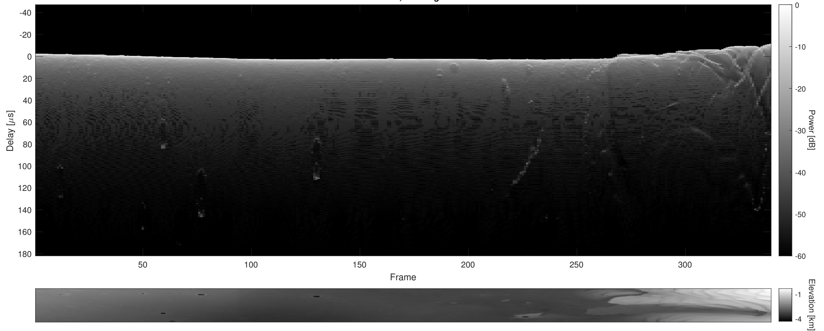
Orbit 20292, Cluttergram
