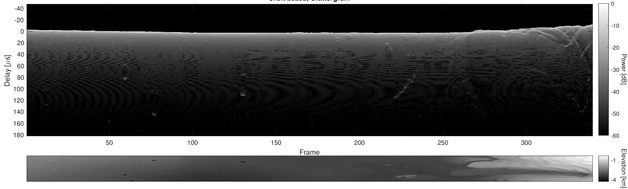
Orbit 20292, Cluttergram
