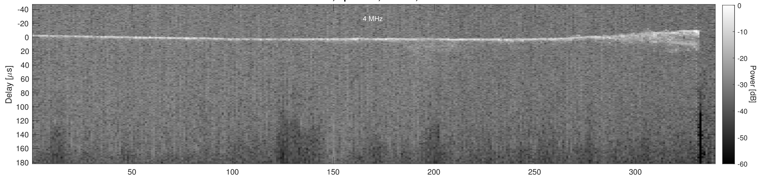
Orbit 20292, Cluttergram
