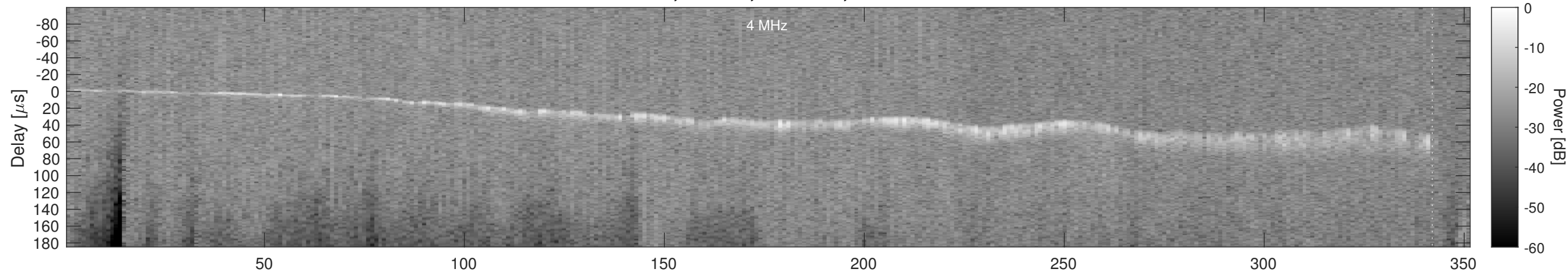
Orbit 20296, Window, Channel 2, Chapman
