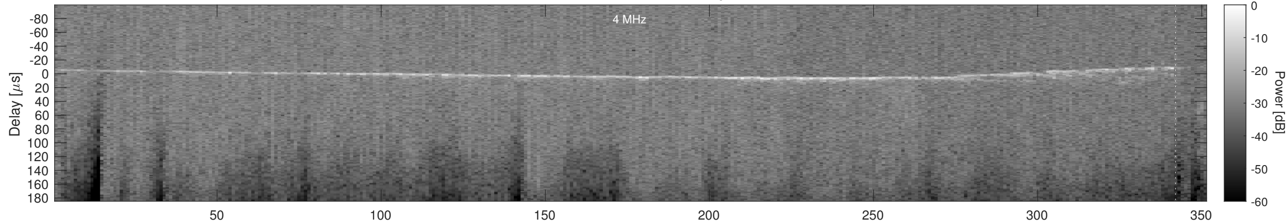
Orbit 20296, Cluttergram
