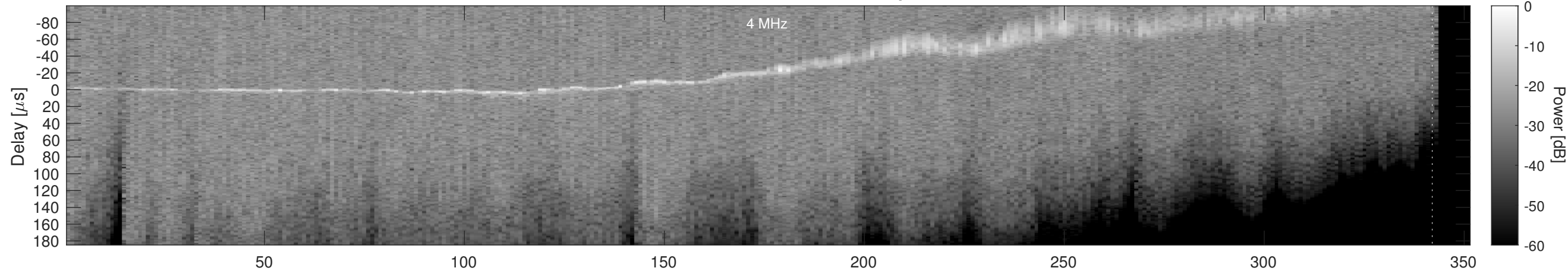
Orbit 20296, Window, Channel 2, Optimized
