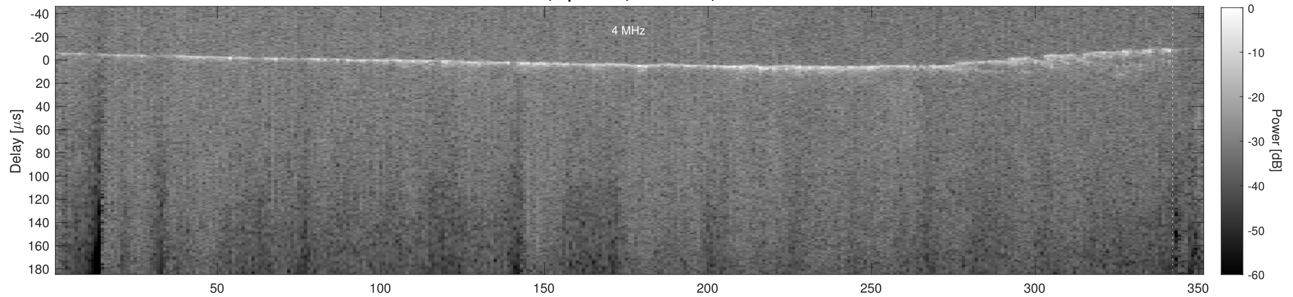
Orbit 20296, Cluttergram
