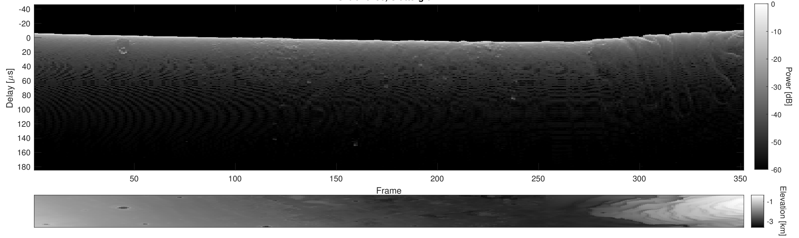
Orbit 20296, Cluttergram
