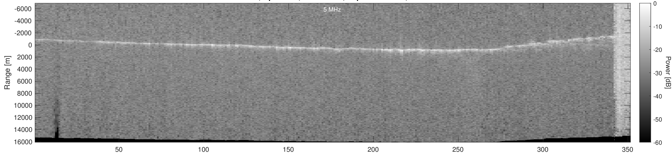
Orbit 20296, Optimized, No Window, Depth-Corrected, Channel 2
