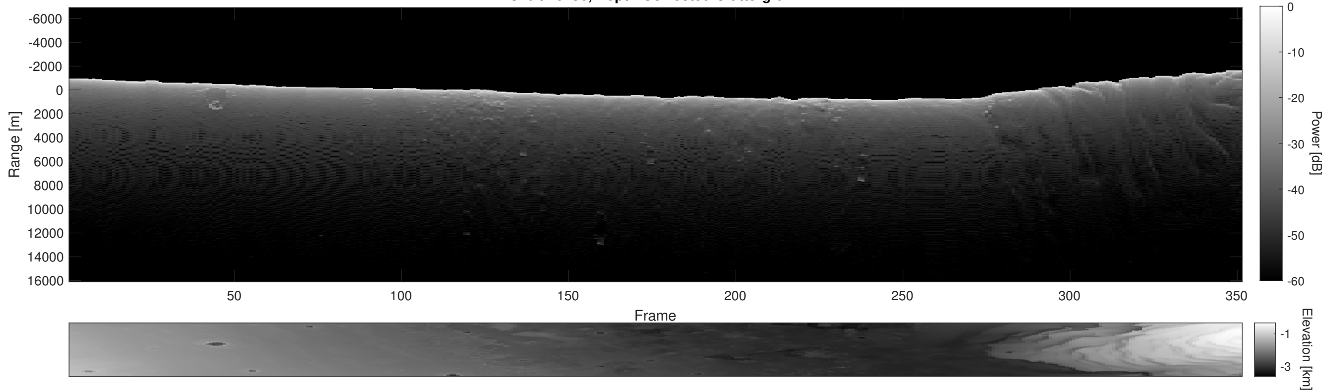
Orbit 20296, Depth-Corrected Cluttergram
