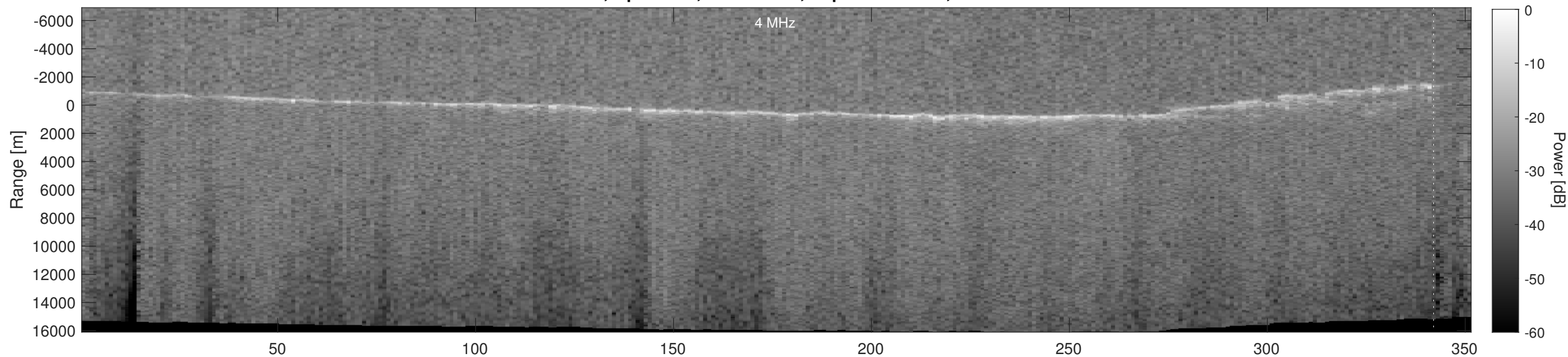
Orbit 20296, Depth-Corrected Cluttergram
