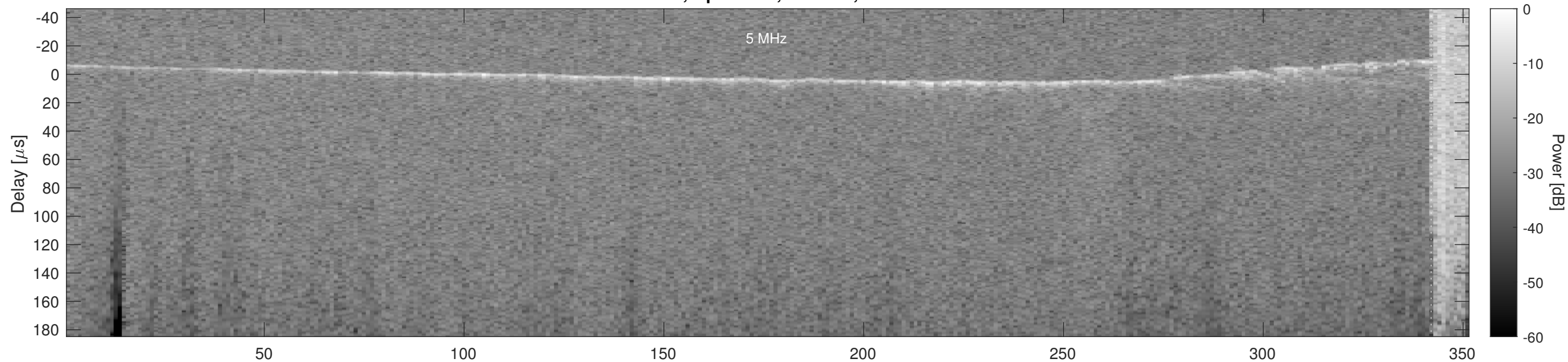
Orbit 20296, Optimized, Window, Channel 2
