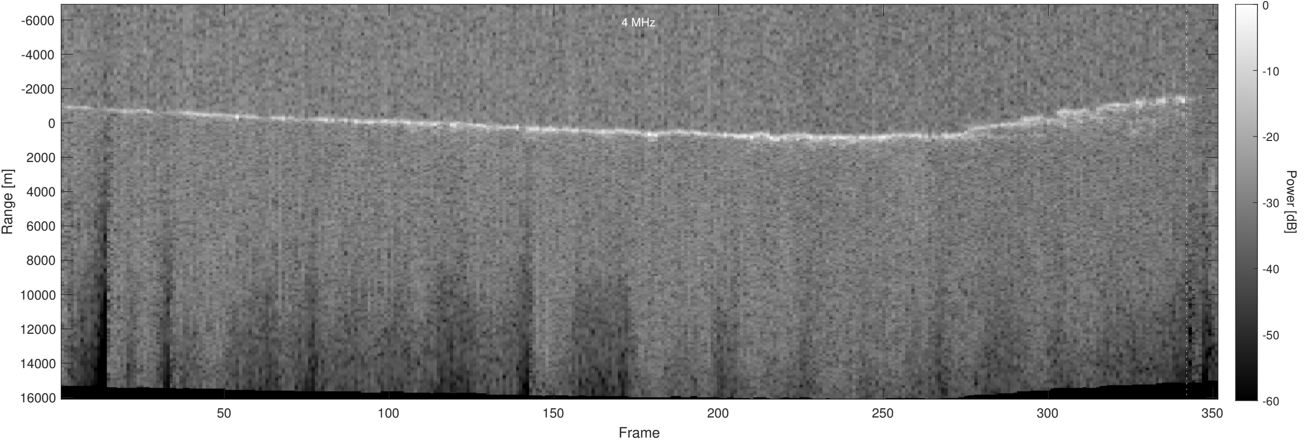
Orbit 20296, Optimized, Window, Depth-Corrected, Channel 2
