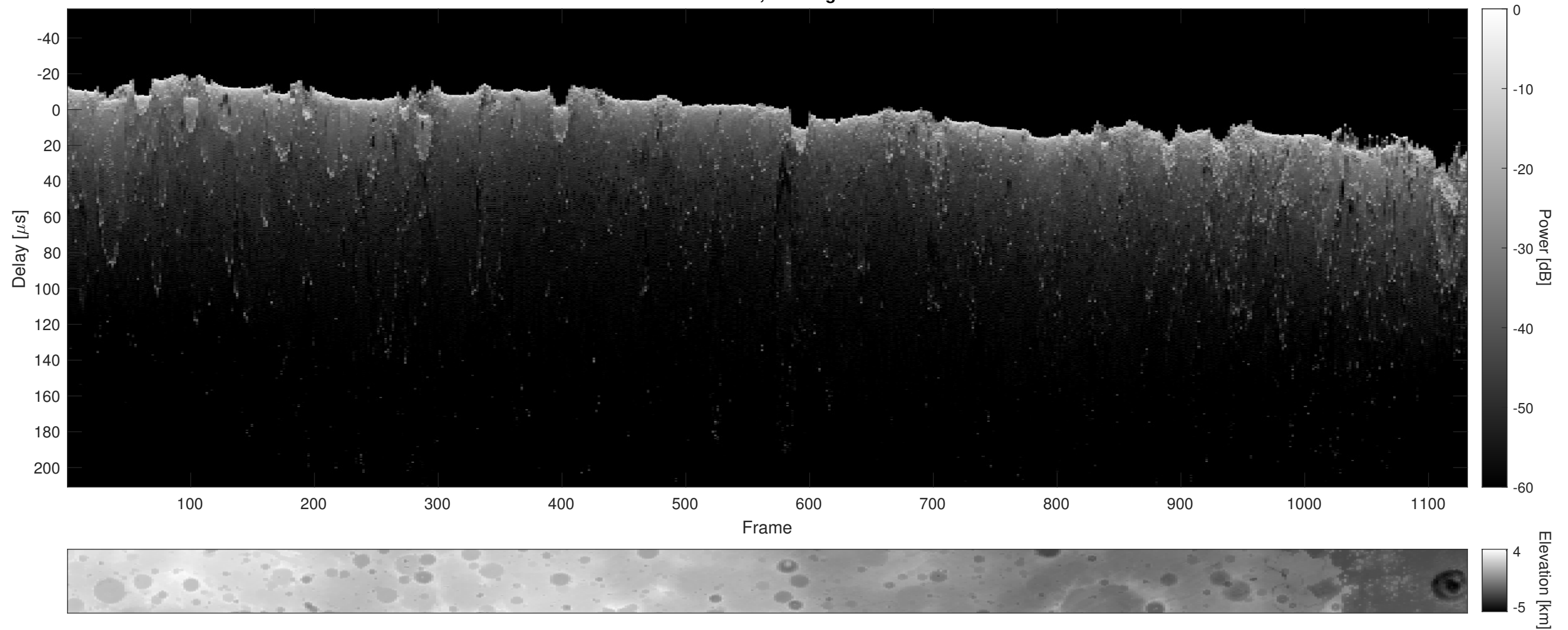
Orbit 20781, Cluttergram
